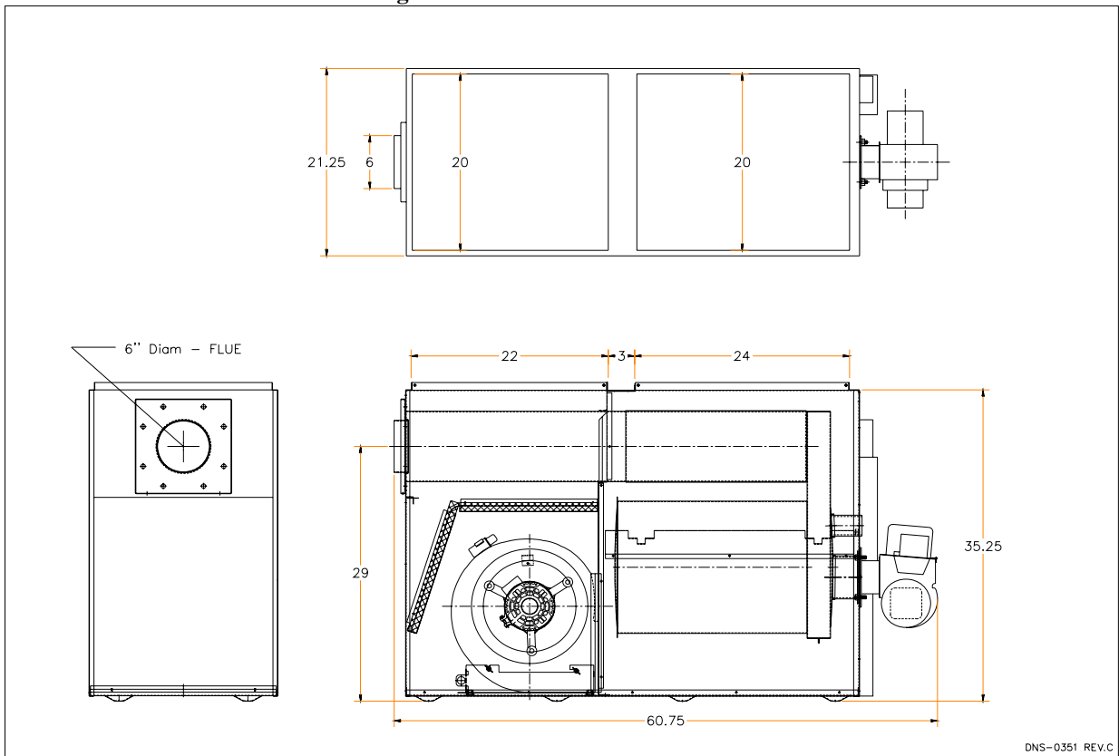
Figure 5: Model AMT2-SM3
