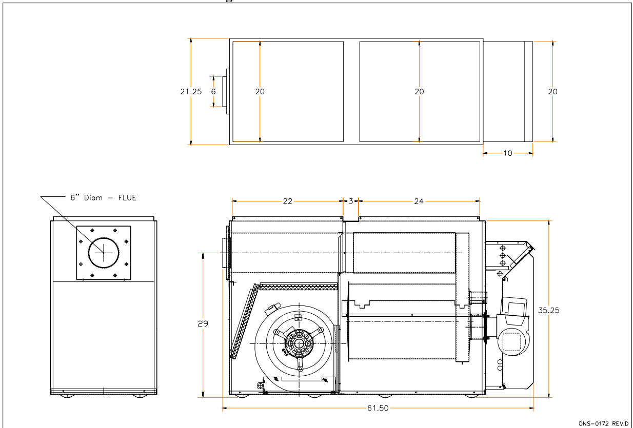
Figure 4: Model AMT2-IM2
